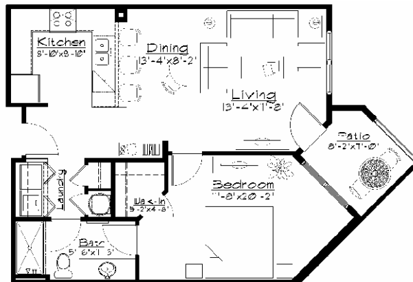
1 BEDROOM/1 BATH WITH LARGE DECK 775 SQ FT TO 785 SQ FT
